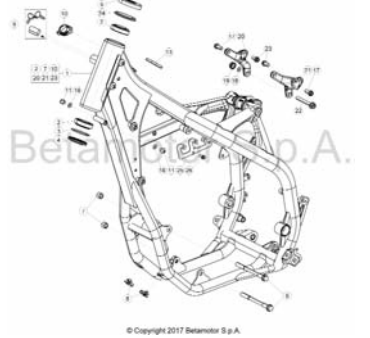
TAV.31 Telaio - Frame - Chassis - Rahmen - Chasis
